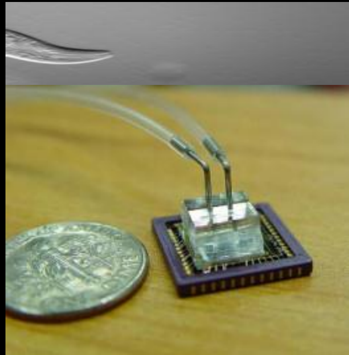
Optofluidic microscope
